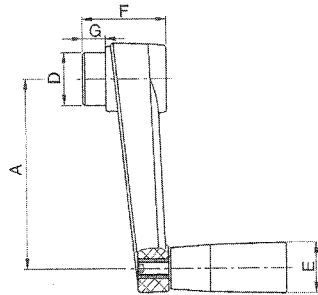
圓孔 Bore
