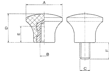
Type A 螺帽 Nut
