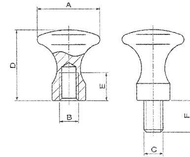
Type A 螺帽 Nut
